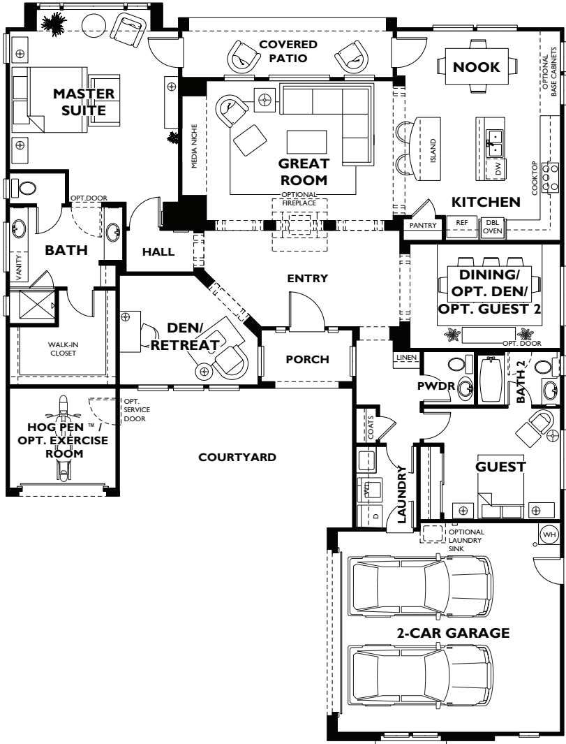
1st Floorplan
