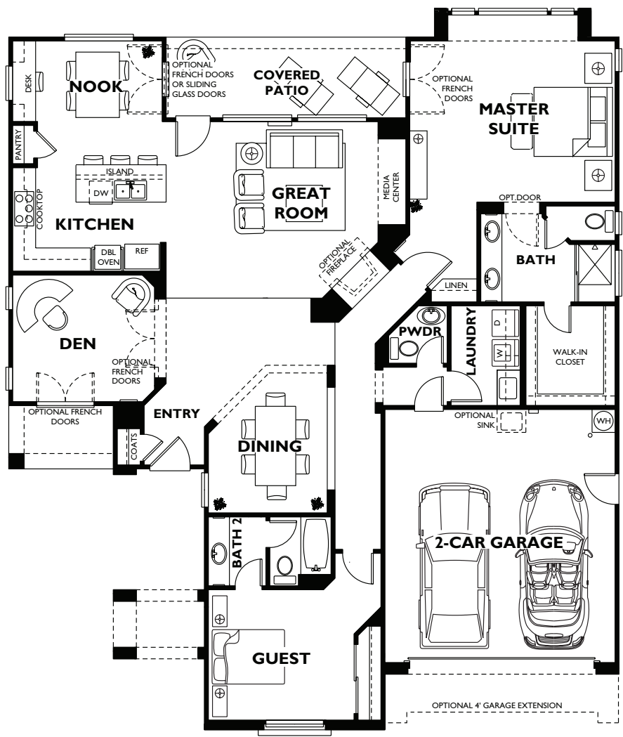
1st Floorplan
