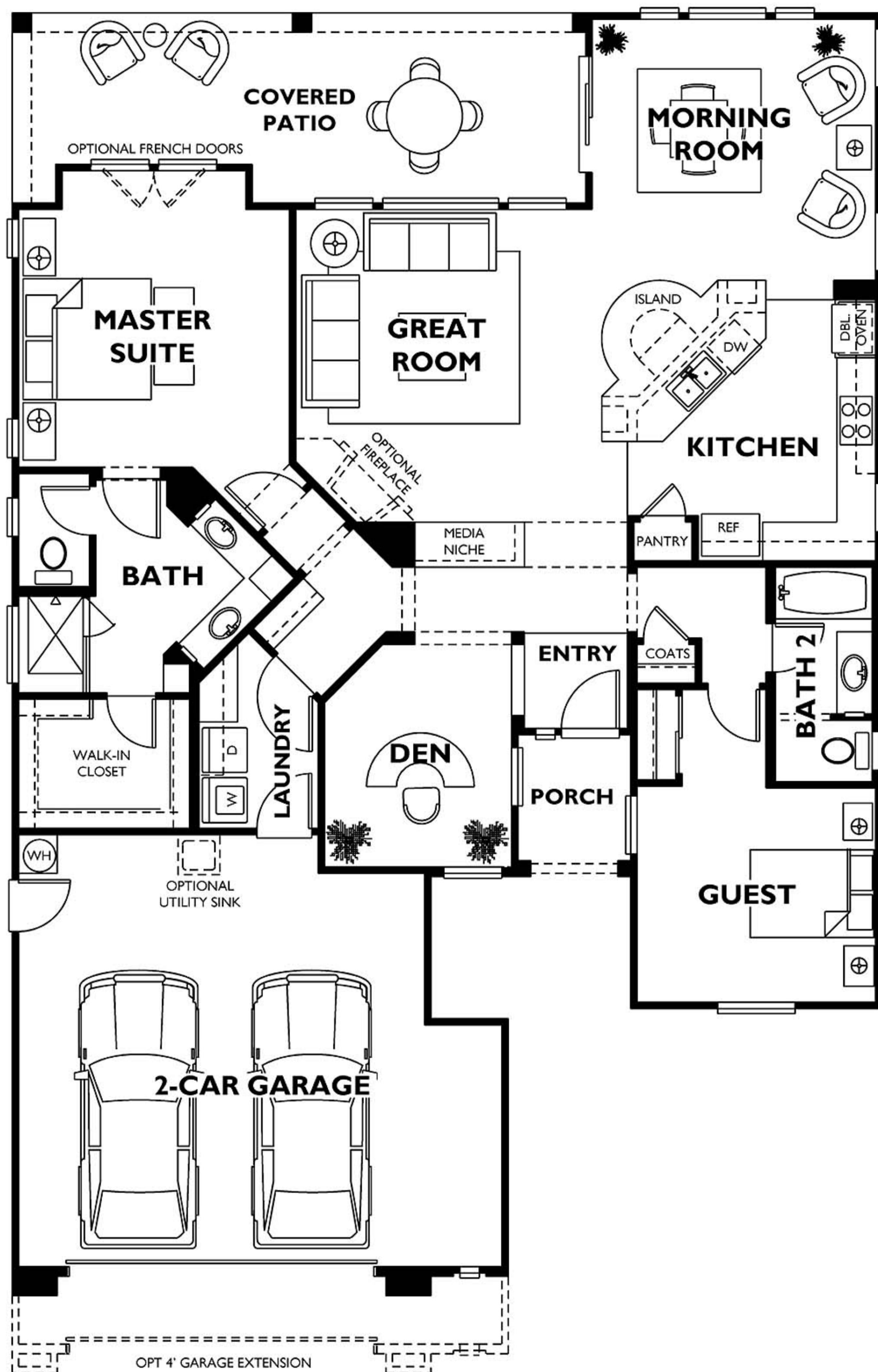
1st Floorplan
