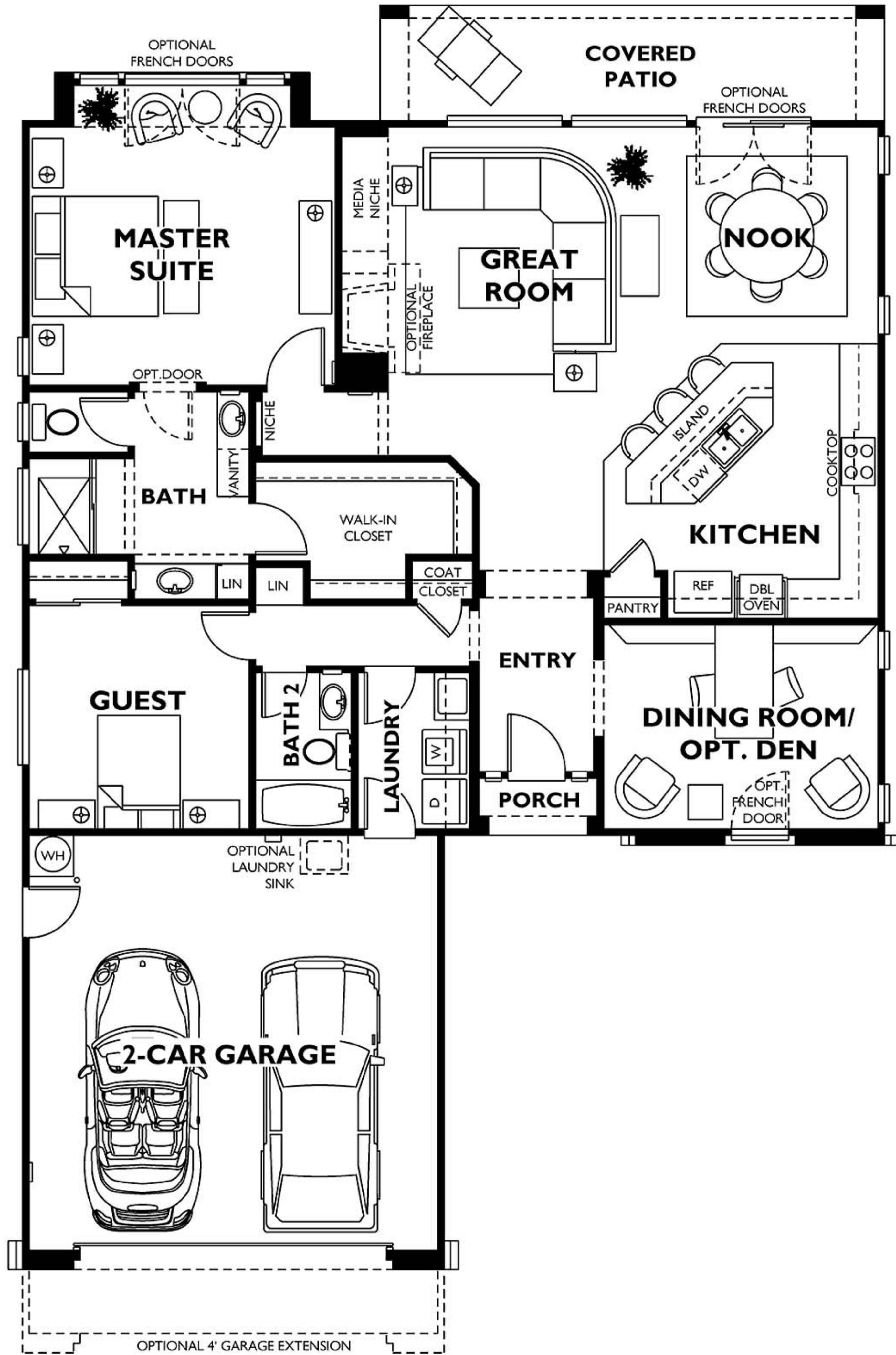
1st Floorplan
